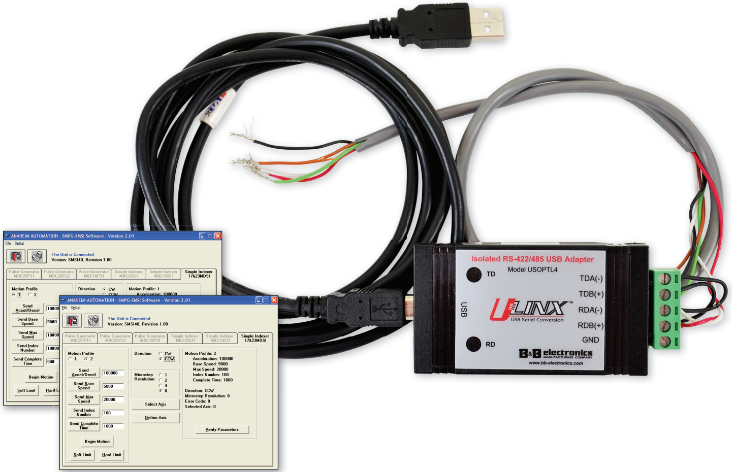
Stepper Motor Programming Software
